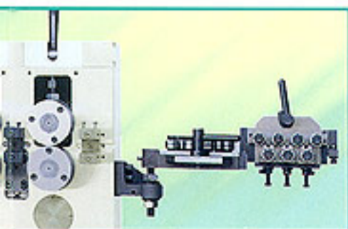
Straightening & straighting unit 直線裝置
